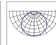
120 = Wide flood 120° 120 = 120° de largura
