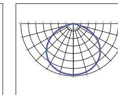
120 = Wide flood 120° 120 = 120° de largura
